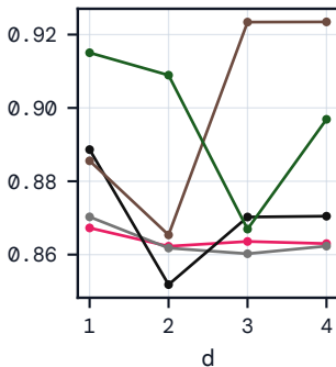
Kendall \tau
